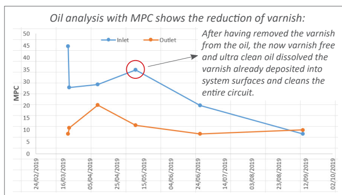
Naturgy, CCC Aceca, Spain with the CJC® VRU Varnish Removal Unit installed
