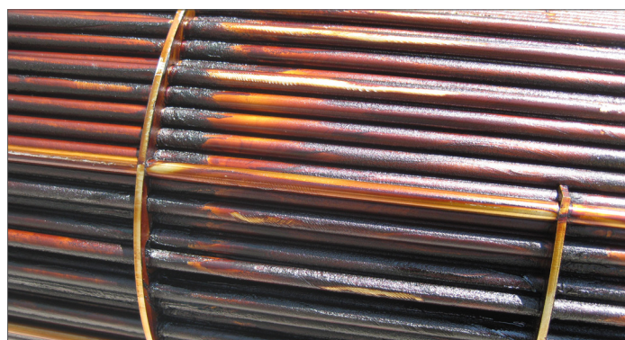
Heat exchanger failure due to varnish build-up on the surface
